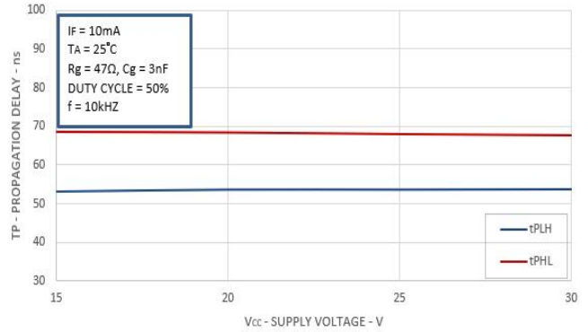
图例 8-传输延时与电源电压曲线图 Fig.8 Propagation Delays vs. VCC
