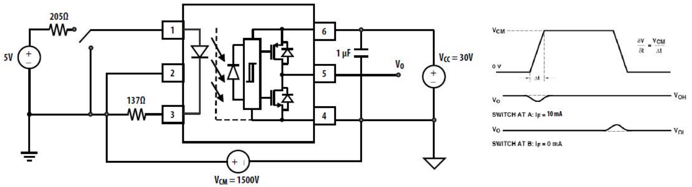
图例 21-共模抑制比测试电路及波形图 Fig.21 CMR Test Circuit with Split Resistors Network and Waveforms
